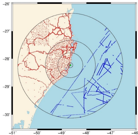
Figure 2 – Distribution of land (in red) and marine (in blue) gravimetric measurements at the IMBT station, Brazil.
